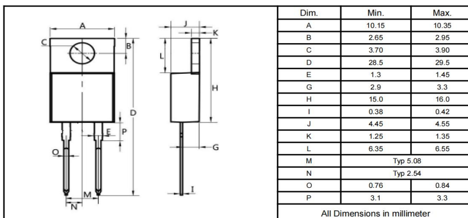
TO-220FAC
